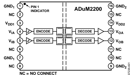
Figure 1. ADuM2200
